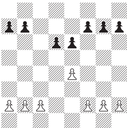
Sicilian - Scheveningen
